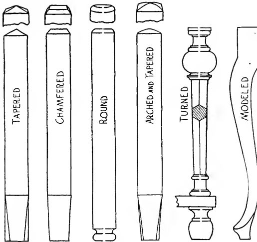
FIG. 386. DETAILS OF POST CONSTRUCTION.
